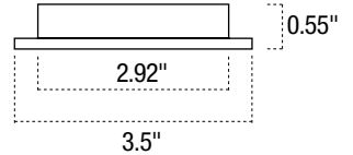
NMPKA-RECBZ: Recess Mount for LED Puck, Bronze NMPKA-RECC: Recess Mount for LED Puck, Chrome NMPKA-RECW: Recess Mount for LED Puck, White
