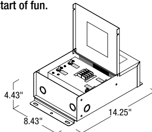
NMT-244/12C2D1: 120/12V 240W C2 Dimm. Driver NMT-244/12C2D1: 277/12V 240W C2 Dimm. Driver
